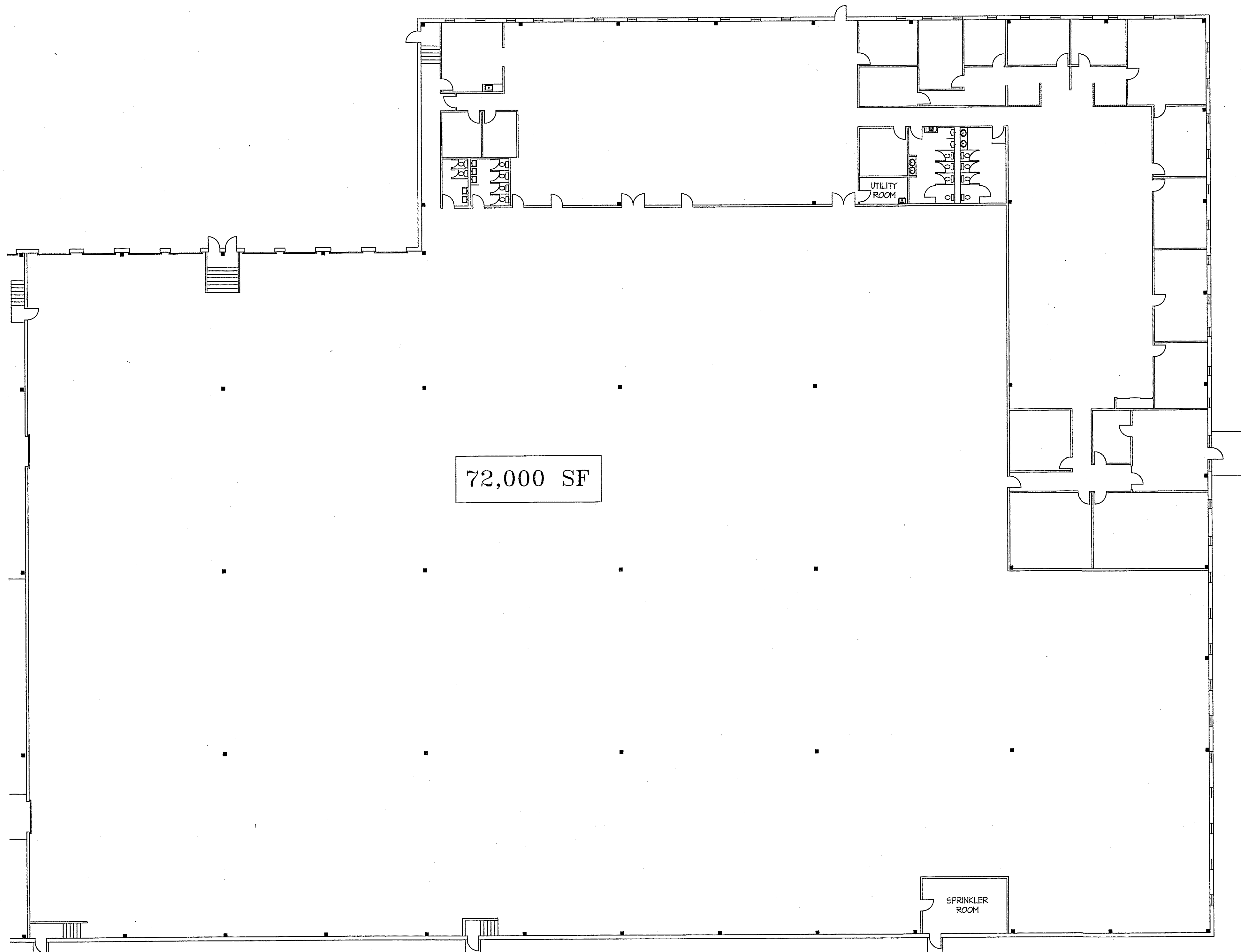
FLOOR PLAN SCALE: 1/16" = 1'-0"
