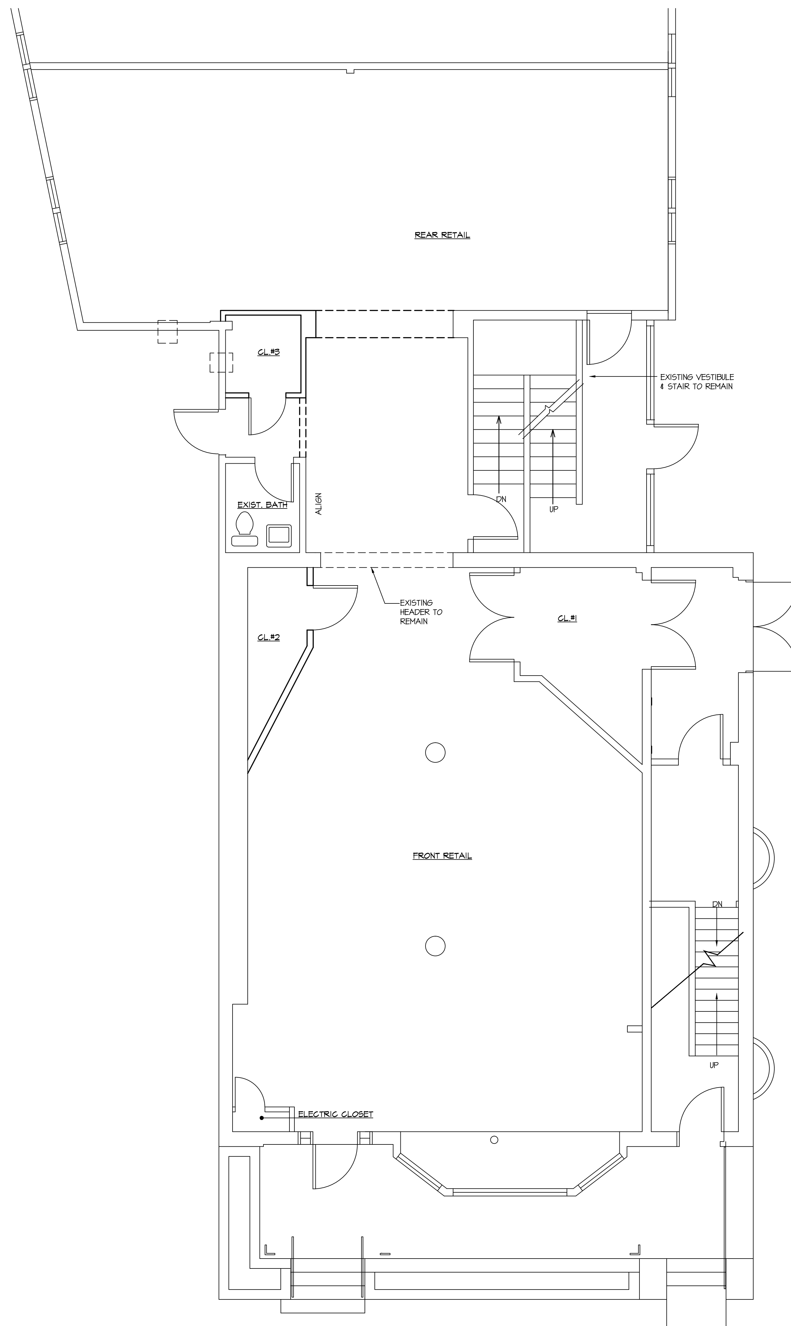
EXISTING 1st FLOOR PLAN SCALE: 1/4" = 1'-0"
